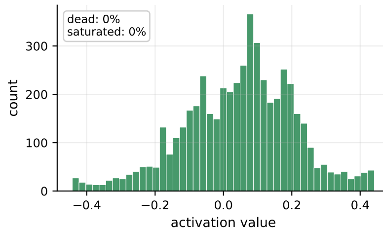
L4 (20 neurons)
