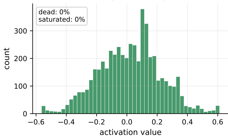
L3 (20 neurons)
