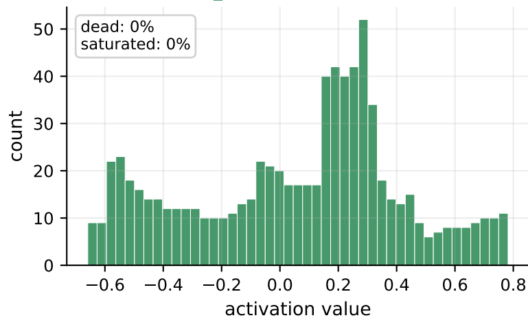
L3 (20 neurons)
