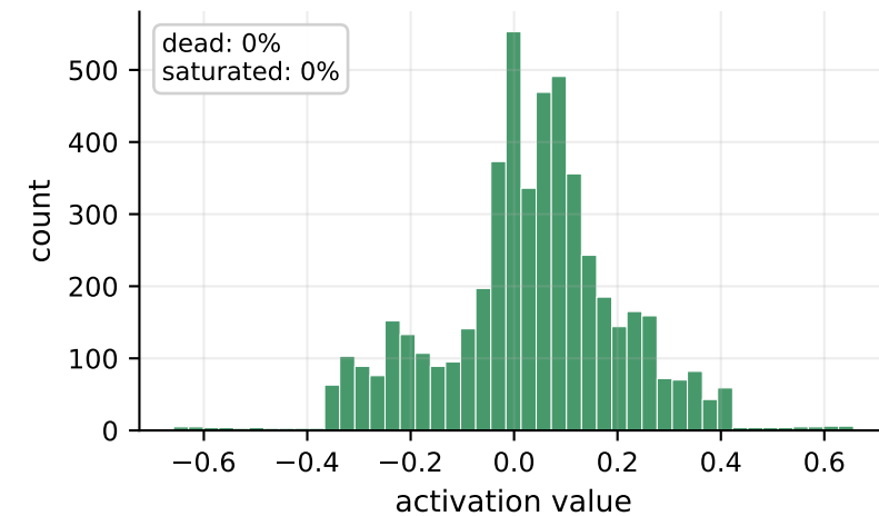
L5 (20 neurons)
