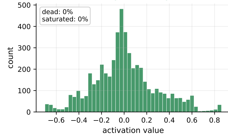
L5 (20 neurons)
