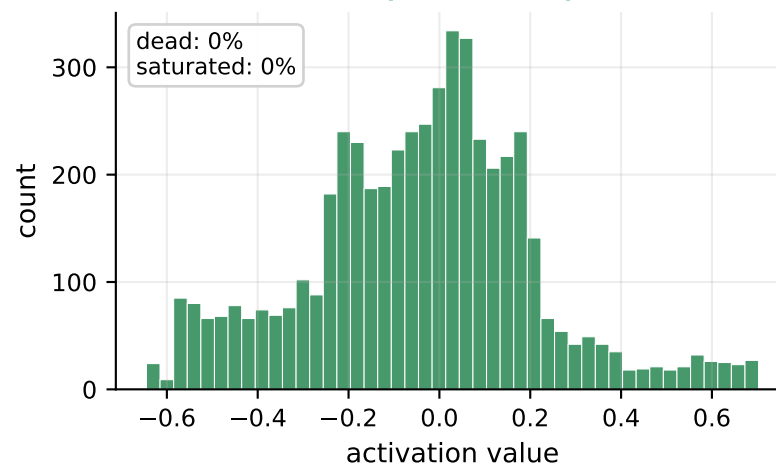
L4 (20 neurons)
